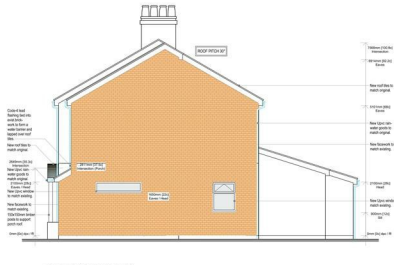
Proposed Side Elevation - (East)
