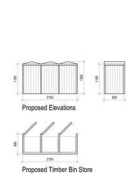
Proposed Elevations
