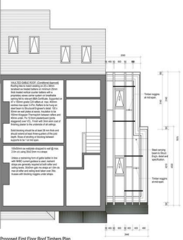
Proposed First Floor Roofing Plan
