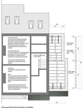
Proposed First Floor Roofing Just Plan
