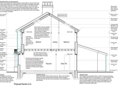
Proposed Section A-A
