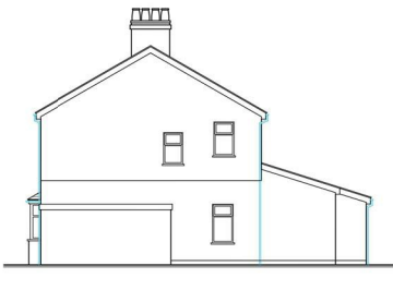
Existing Side Elevation - (East)
